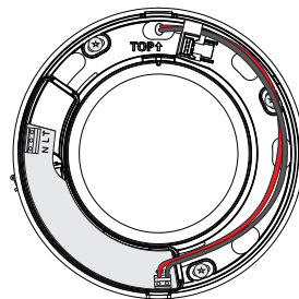
L. 12 V DC connection
