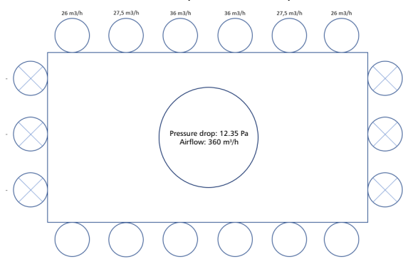
0-6-0-6 (200 mm inlet)
