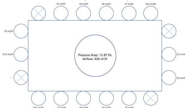
2-5-2-5 (200 mm inlet)
