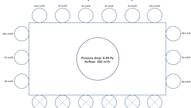
3-6-3-0 (200 mm inlet)
