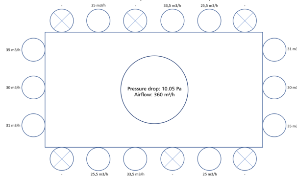
3-3-3-3 (200 mm inlet)
