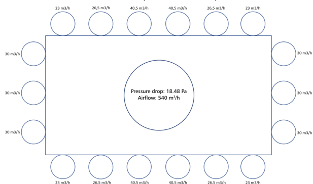
3-6-3-6 (200 mm inlet)
