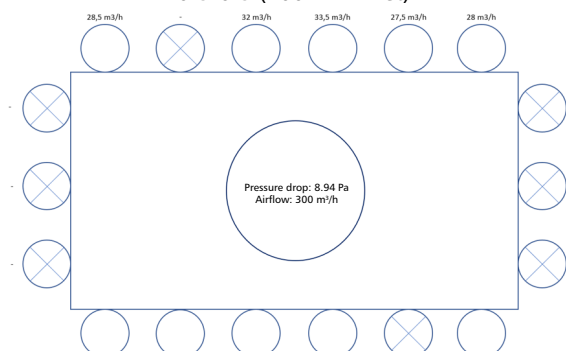
0-5-0-5 (200 mm inlet)
